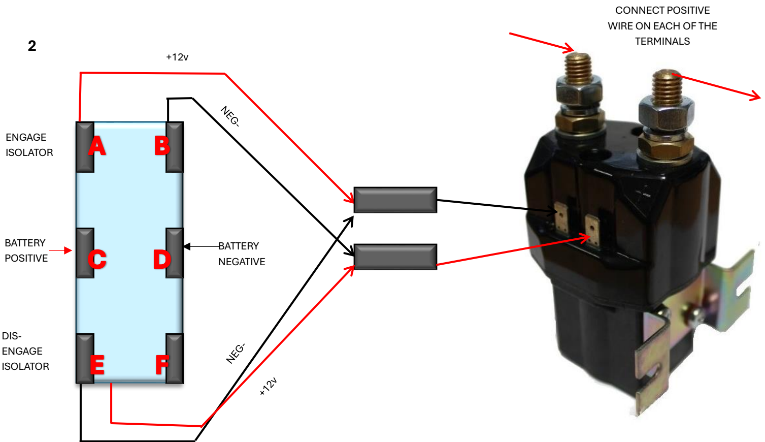
Wiring Diagram
